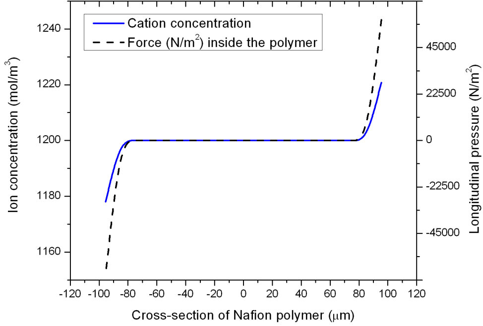
Figure 3. Cation distribution in charge balance state. Also longitudinal force according to modeling inside the polymer is shown. Notice that force grows faster near the boundaries of the polymer than cation distribution. The reason for that is quadratic term in force formula as shown in Equation 3. It is important to notice that the graph is somehow illustrative because real simulation maximum values for concentration and specially for stress are larger.
